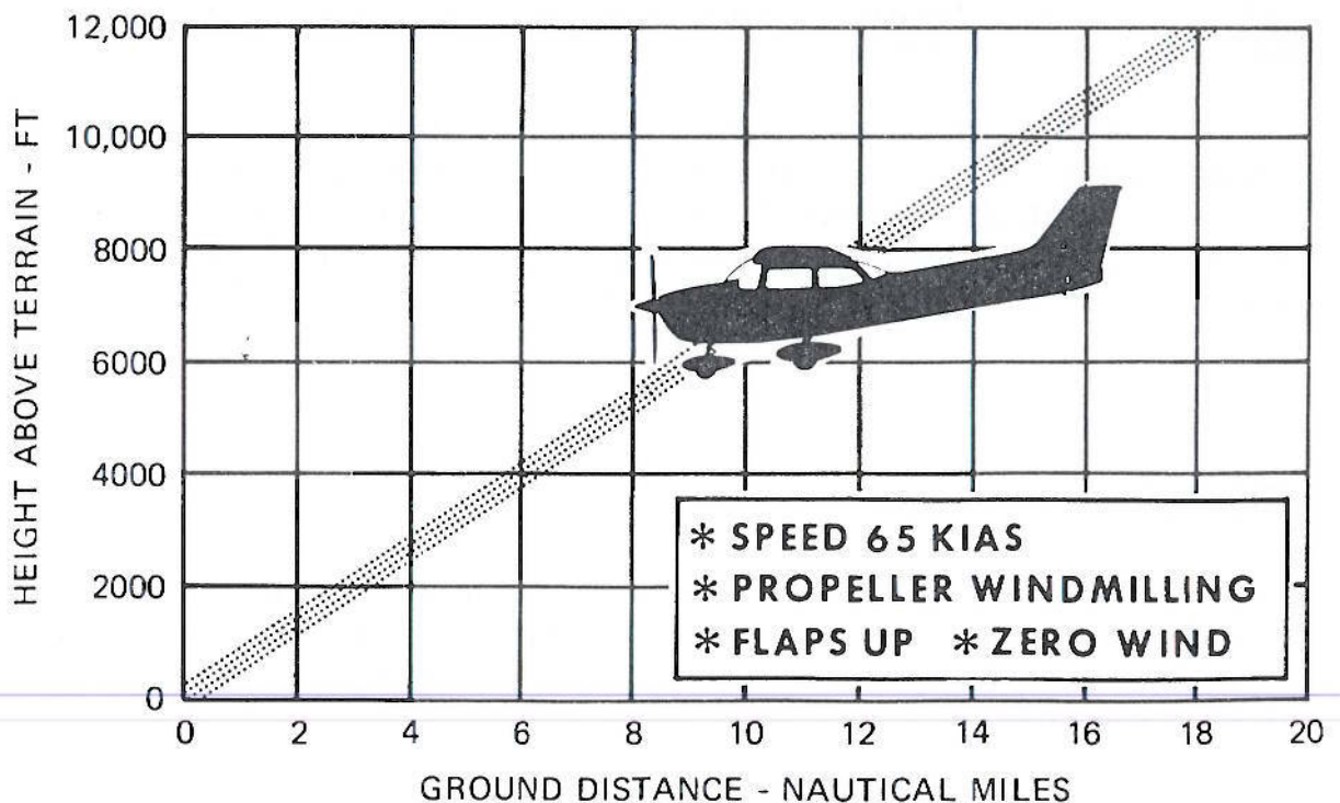
Figure 3-1. Maximum Glide
